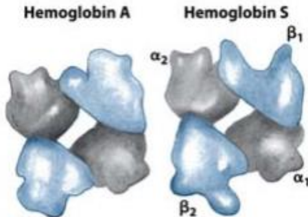
Figure 1-23a Comparison of Hemoglobin A and Hemoglobin S. © 2009 W. H. Freeman and Company
