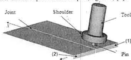
Figure 1. Tool and work pieces before welding [8]
