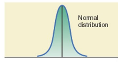
(e) Sampling distribution of \bar{x} for n = 100 .
