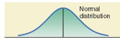
(b) Sampling distribution of \bar{x} for n = 5 .
