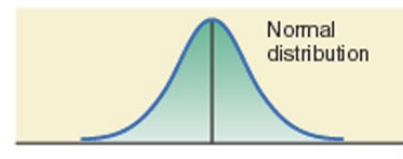
(c) Sampling distribution of \bar{x} for n = 16 .
